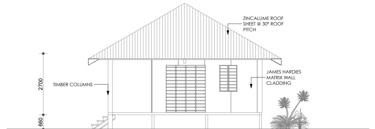
ELEVATION 4 Scale 1:100
