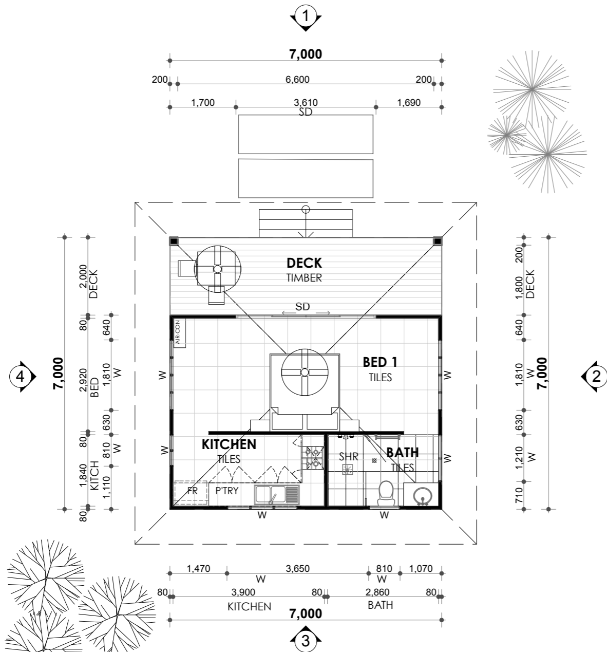
SKETCH PLAN Scale 1:100
