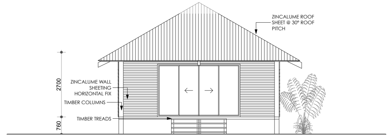
ELEVATION 1 Scale 1:100
