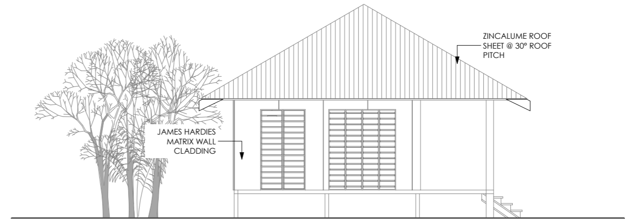
ELEVATION 2 Scale 1:100
